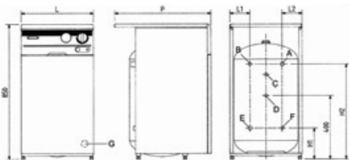
LUNA UB 80-120 / SLIM UB 80 - 120
