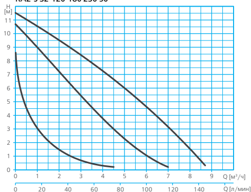
RA2-S 32-120-180 230 50
