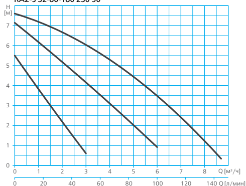
RA2-S 32-80-180 230 50
