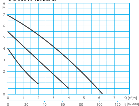
RA2-S 32-70-180 230 50
