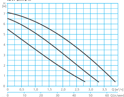
RA1-S...70 ...
