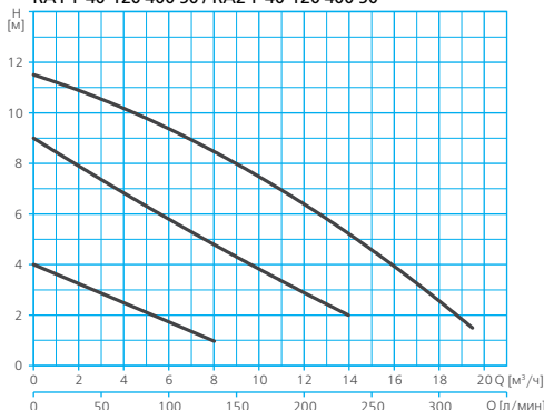
RA1-F 40-120 400 50 / RA2-F 40-120 400 50
