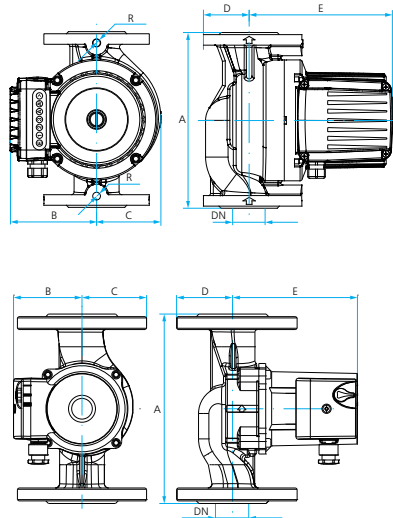
RA2-S
