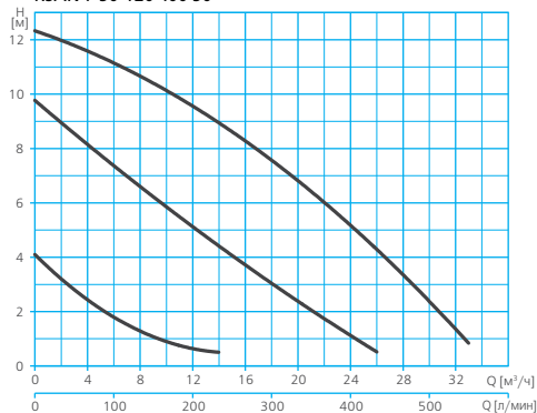
RSAN-F 50-120 400 50
